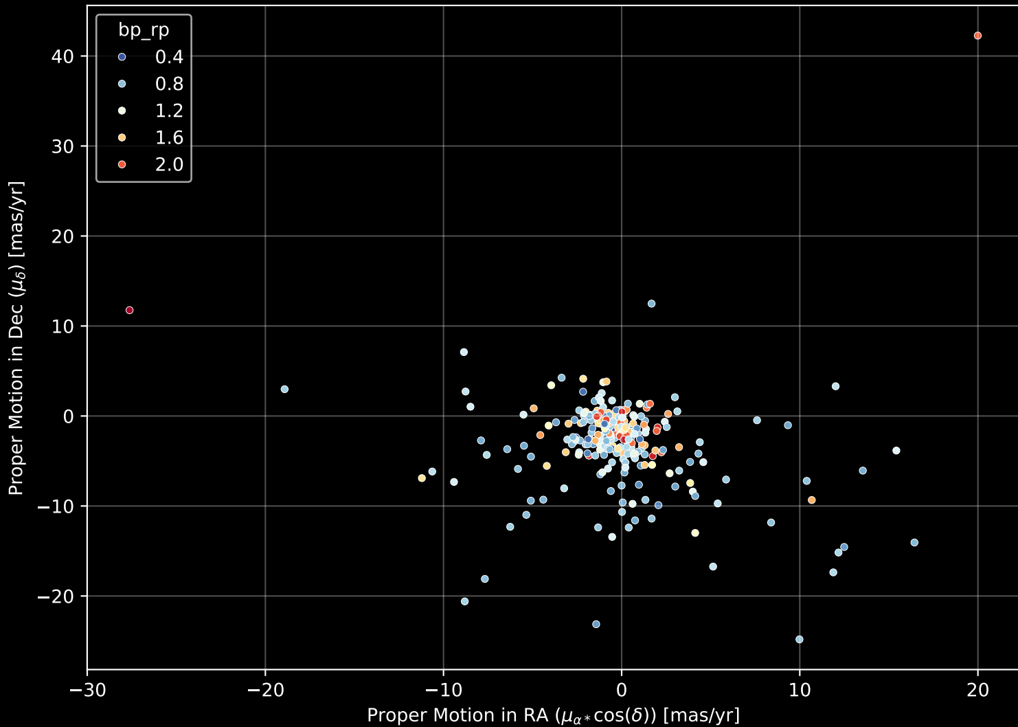
GALAH DR4 Field: [9473] Proper Motion Diagram (n= 276)
