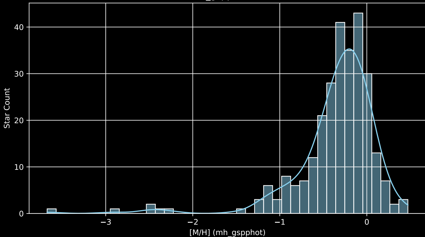
GALAH DR4 Field: [9473] [M/H] (mh_gspphot) (n= 275)
