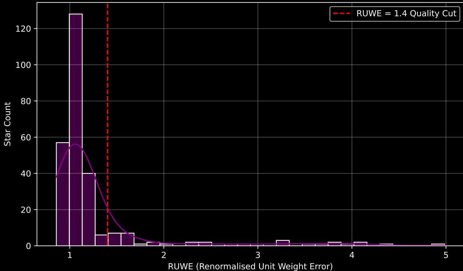
GALAH DR4 Field [9473] RUWE Distribution (n= 268)
